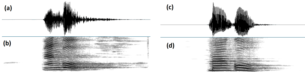
Fig. 3: Waveform and spectrogram of a same word ( mango ) pronounced by a child with ASD (a,b) and a normal child (c, d). The differences in F0 and Formants frequencies values are clearly understandable between a ASD and normal child. The Y-axis varies from 0 Hz to 5000 Hz in the case of the spectrograms.
